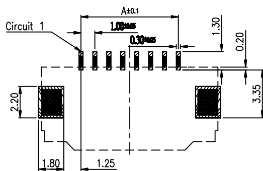
RECOMMENDED PC BOARD PATTERN DIM.(REF.)
